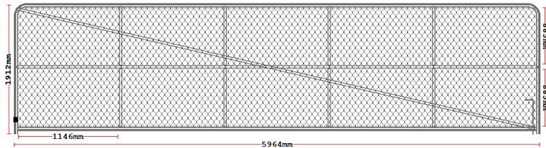
Plain Top Single Leaf Left Hinge Gate 6000mm Opening Size
